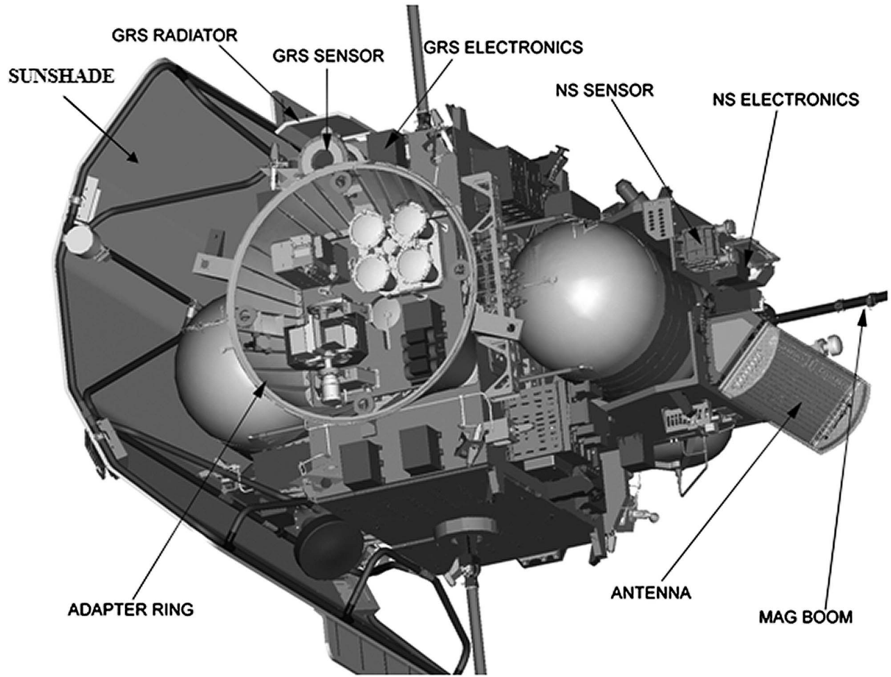
Figure A3. CAD drawing of GRS and NS as positioned on the MESSENGER spacecraft. Only a portion of the 3.6-m boom for MESSENGER's Magnetometer (MAG) is shown. Also indicated are one of MESSENGER's two high-gain phased-array antennas, the carbon fiber sunshade, and the adapter ring by which the spacecraft was mated to the upper stage of the launch vehicle. Figure reproduced from Rhodes et al. [2011].
