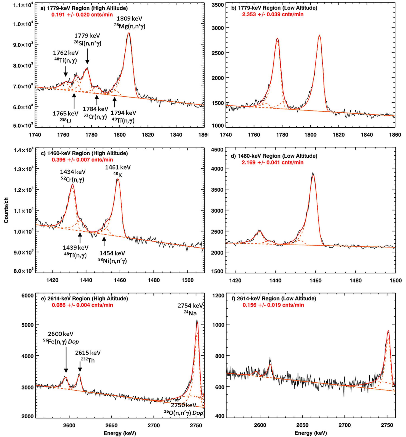
Figure 4. High- and low-altitude peak fits for near-nadir ( \theta_n \leq 15^\circ ) GRS measurements of the (a and b) 1779-keV Si, (c and d) 1461-keV K, and (e and f) 2615-keV Th gamma rays as well as neighboring and interfering peaks that are included to ensure good fits to the entire region. Peak energies and sources are listed in the high-altitude spectra (Figure 4, Left) and are based on the identifications by Evans et al. [2006]. Dop indicates the peak is Doppler broadened.
